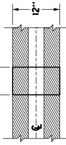
RUMBLE STRIP DETAIL
